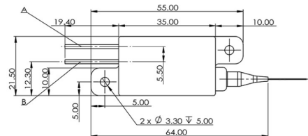
Large form factor coupled in a 105 \mu\text{m} fiber
