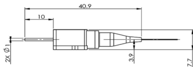
Small form factor coupled in a 200 \mu\text{m} fiber (specifications may vary for this model)
