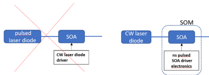
Figure 8 : SOA, when driven with specific electronics, behaves like a fiber modulator with no insertion loss (SOM)
