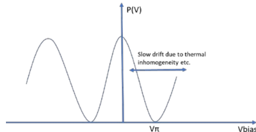
Figure 5 : Transfer function of an intensity modulator
