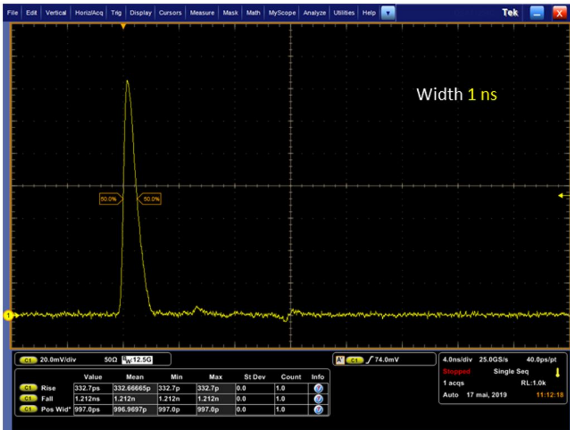
Figure 11b: 1 ns pulse obtained at 1064 nm with AeroDIODE SOM-std.
